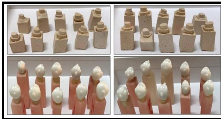
(Figure 6): Design of the crown using Cercon CAD/CAM
